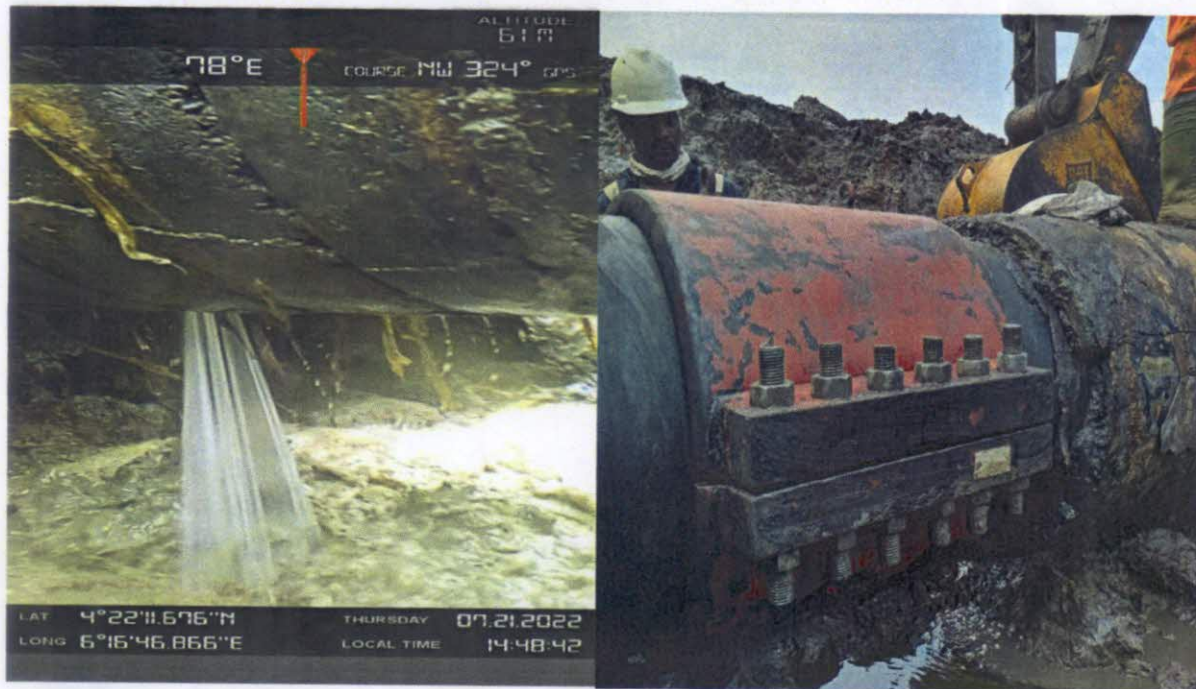
PICTURE A: CORROSION AT 6 O' CLOCK POSITION. PICTURE B: CLAMPED SECTION OF THE PIPELINE.
